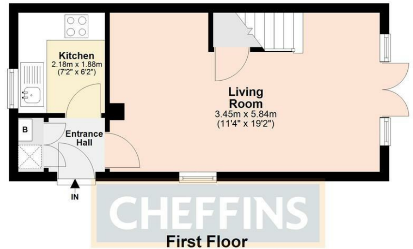
First Floor Approx. 27.0 sq. metres (290.7 sq. feet)
